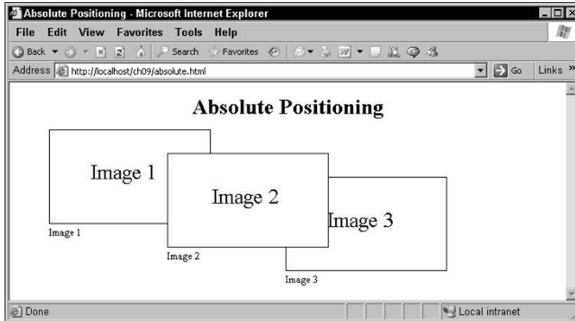
Figure 9-9: Setting z- index to customize overlapping.
